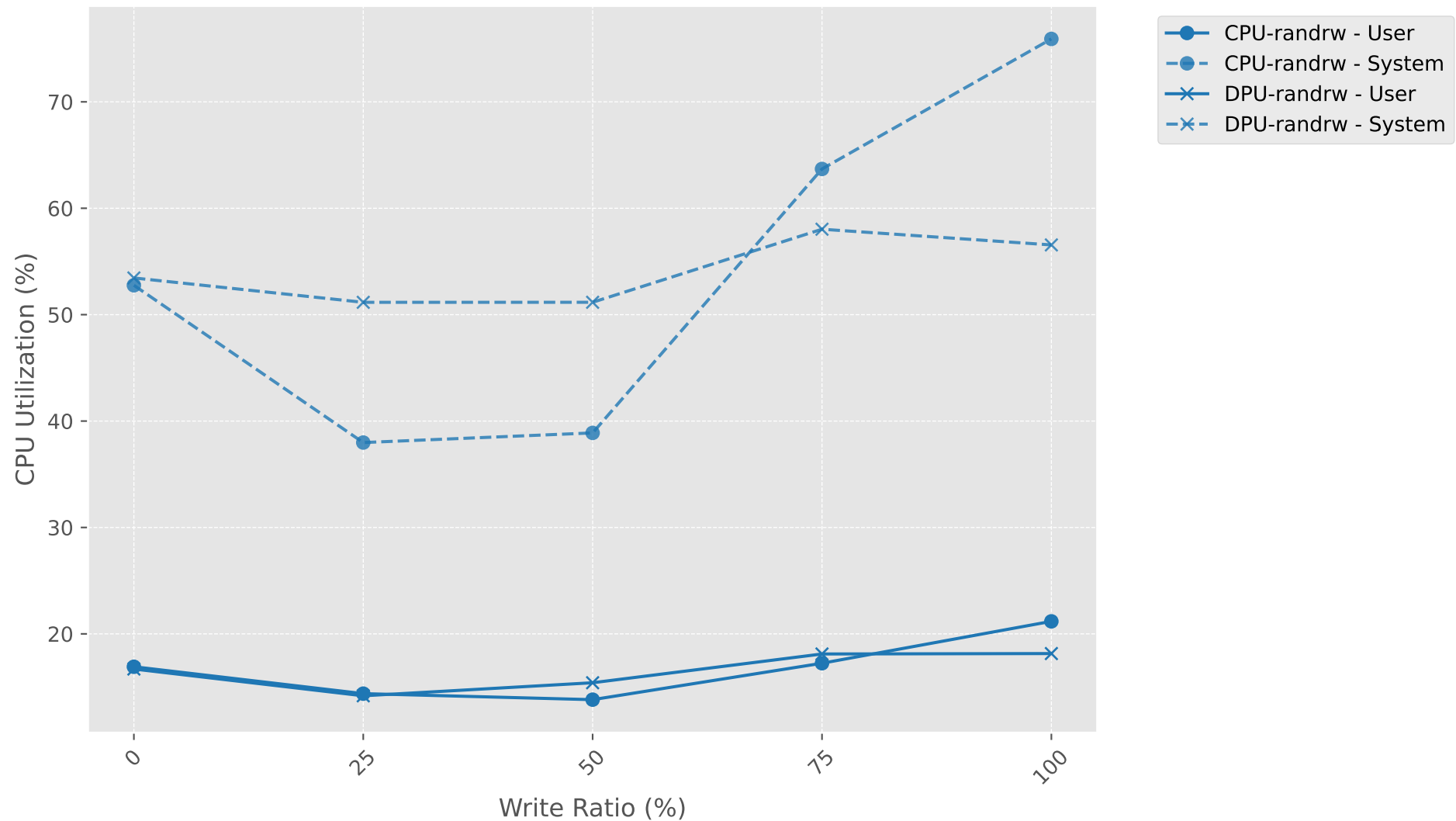
CPU Utilization vs Write Ratio (rwmixwrite-4k-8)
